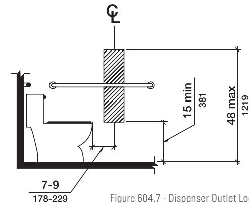
Figure 604.7 - Dispenser Outlet Location
